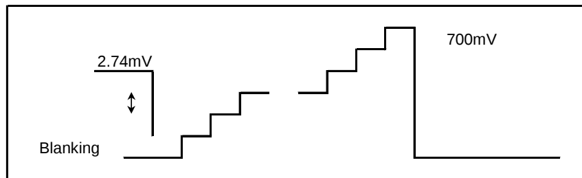
Fig. 3.01 - Video Signal
