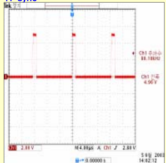
H-sync
