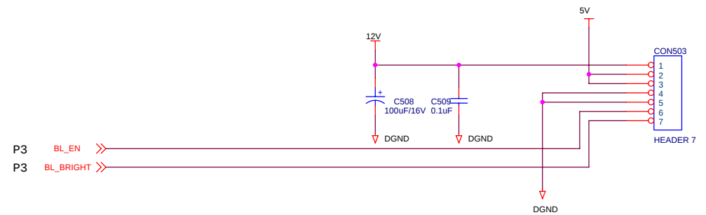
Back Light Connector
