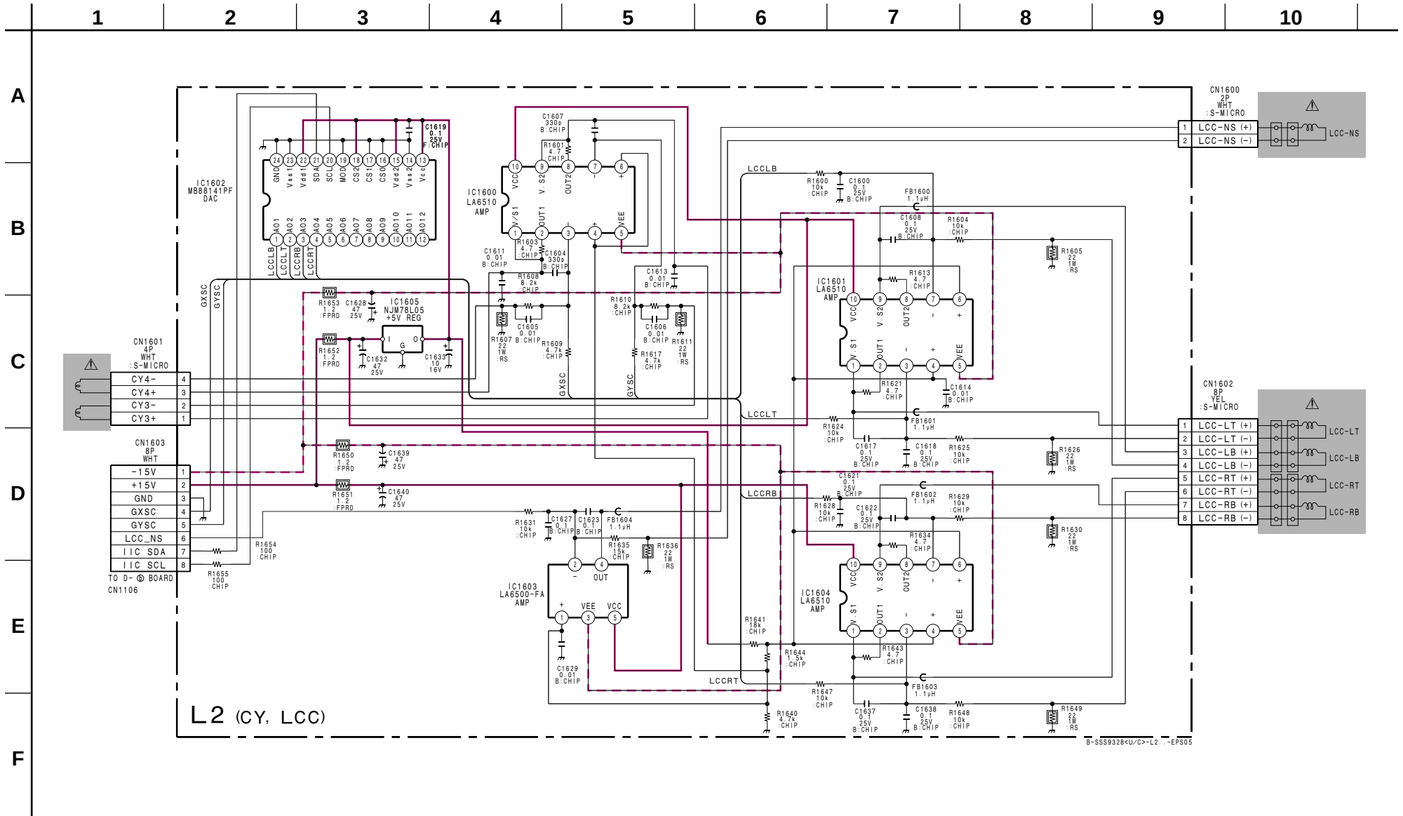
(5) Schematic Diagram of L2 Board
